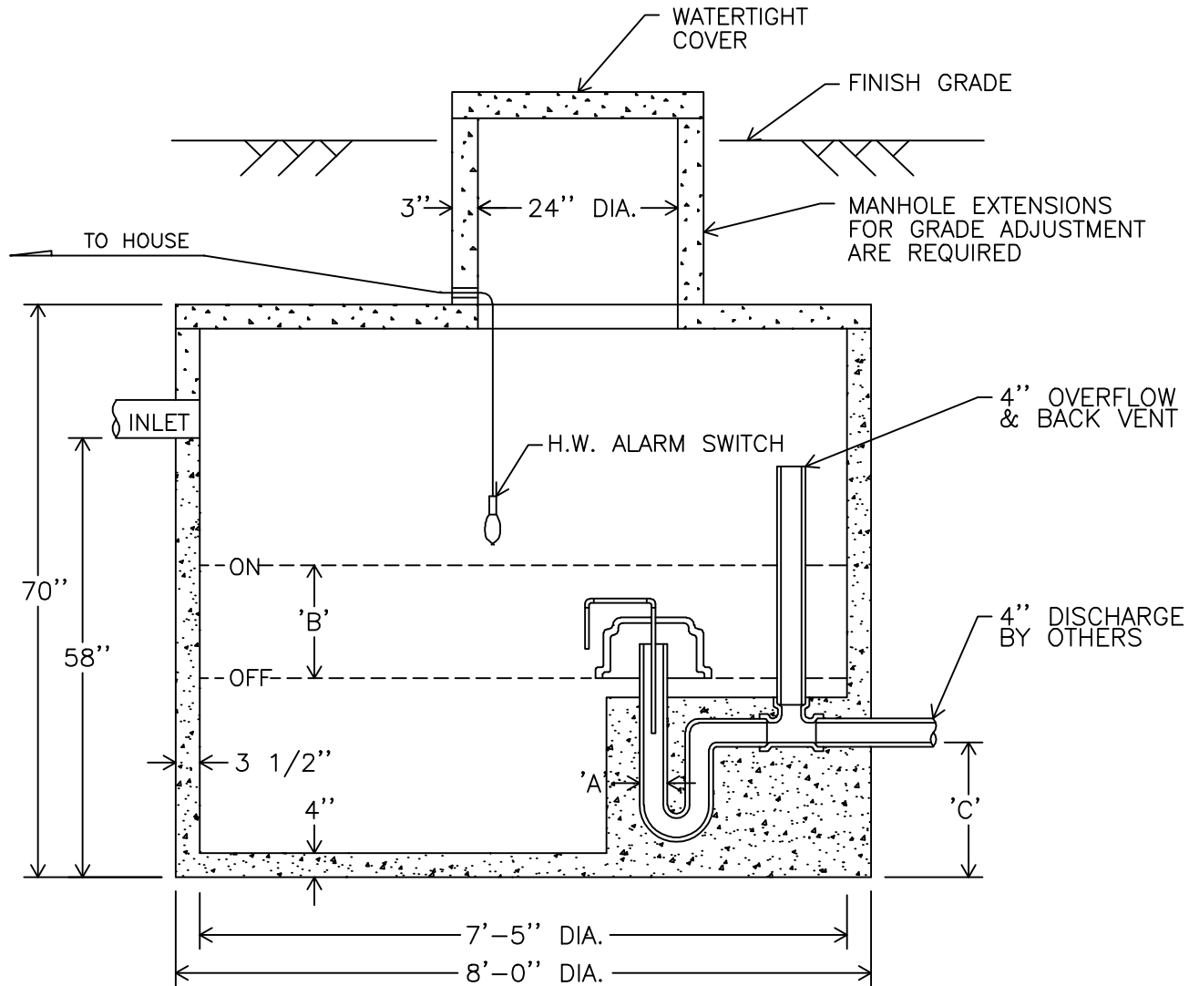
DIMENSION TABLE
