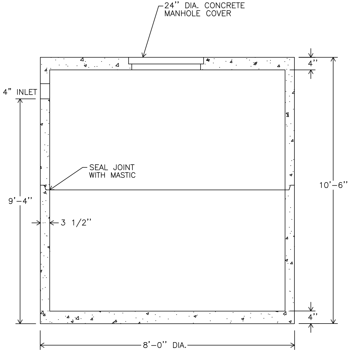
-SECTION ELEVATION-
