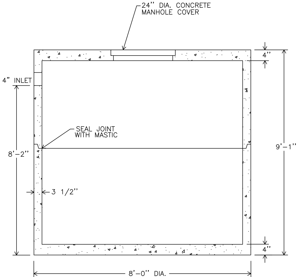
-SECTION ELEVATION-
