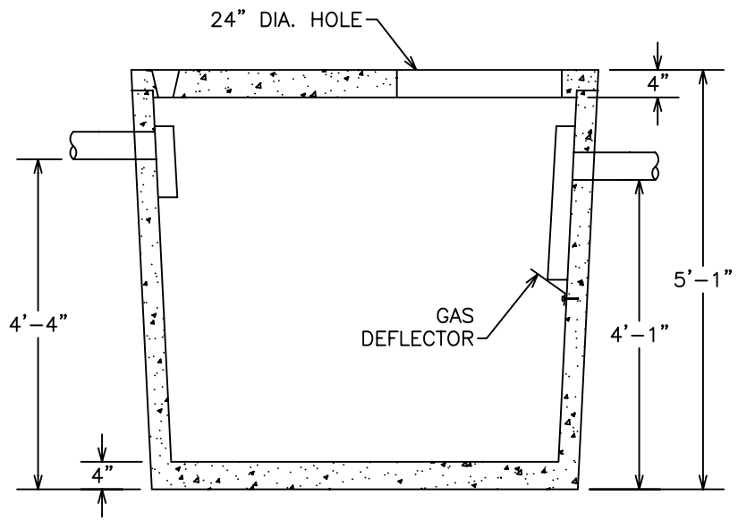
—SECTION—
