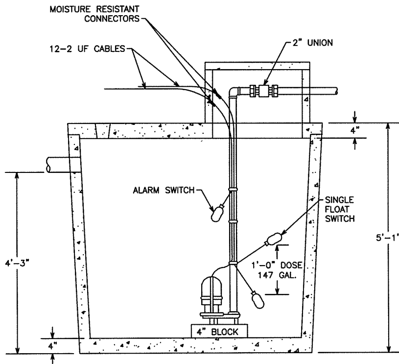
-SECTION-
