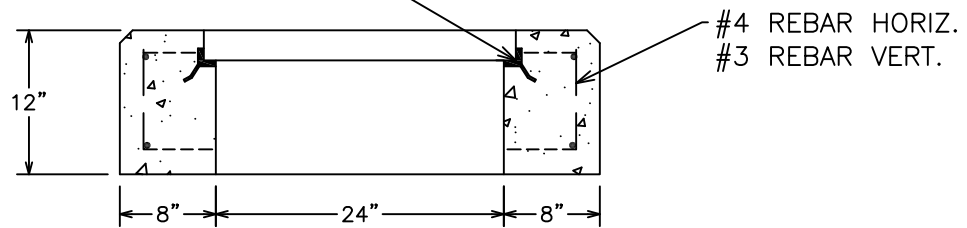
-SECTION-
