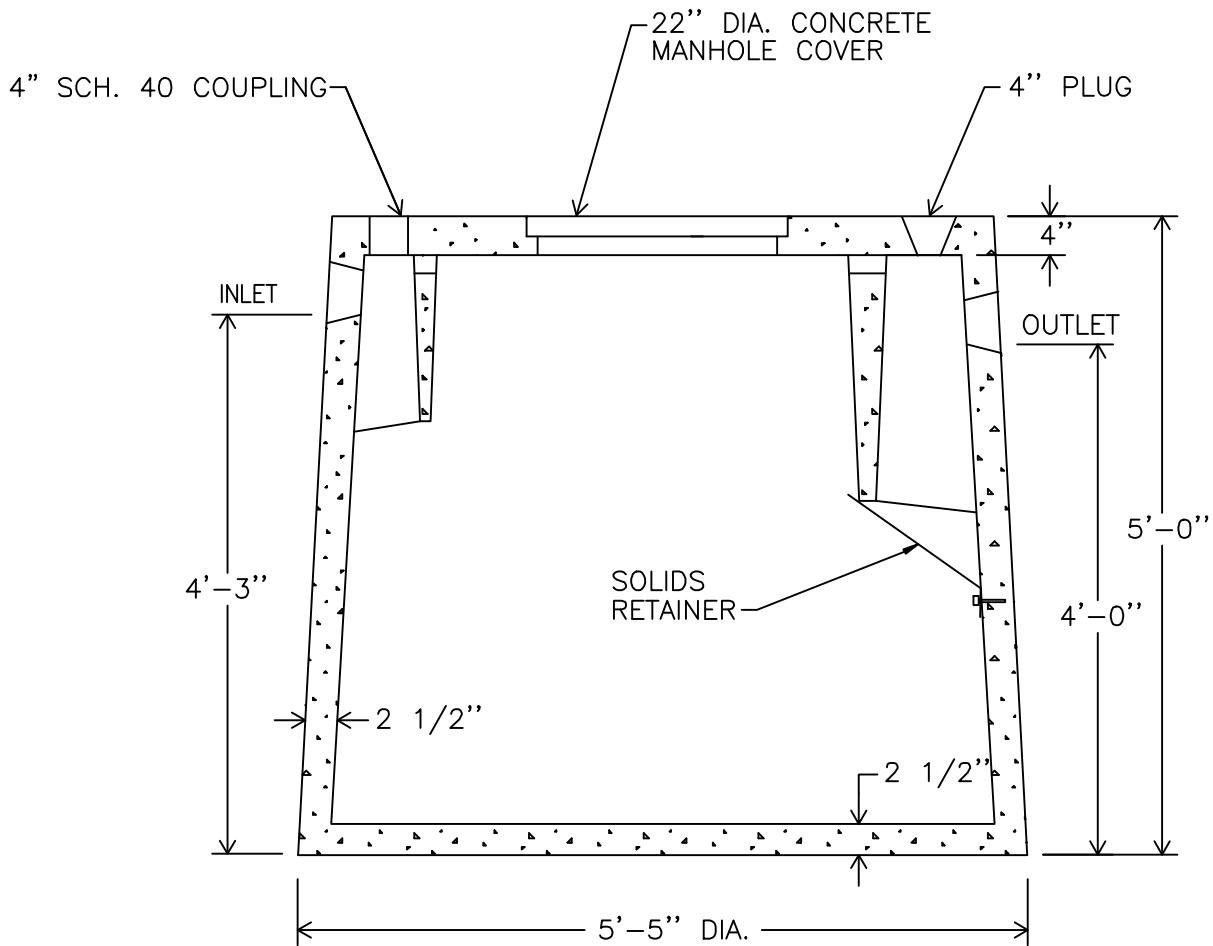
-SECTION ELEVATION-
